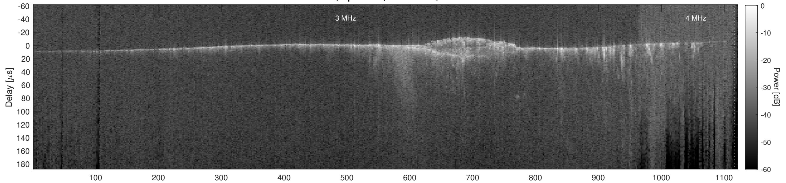
Orbit 14035, Cluttergram
