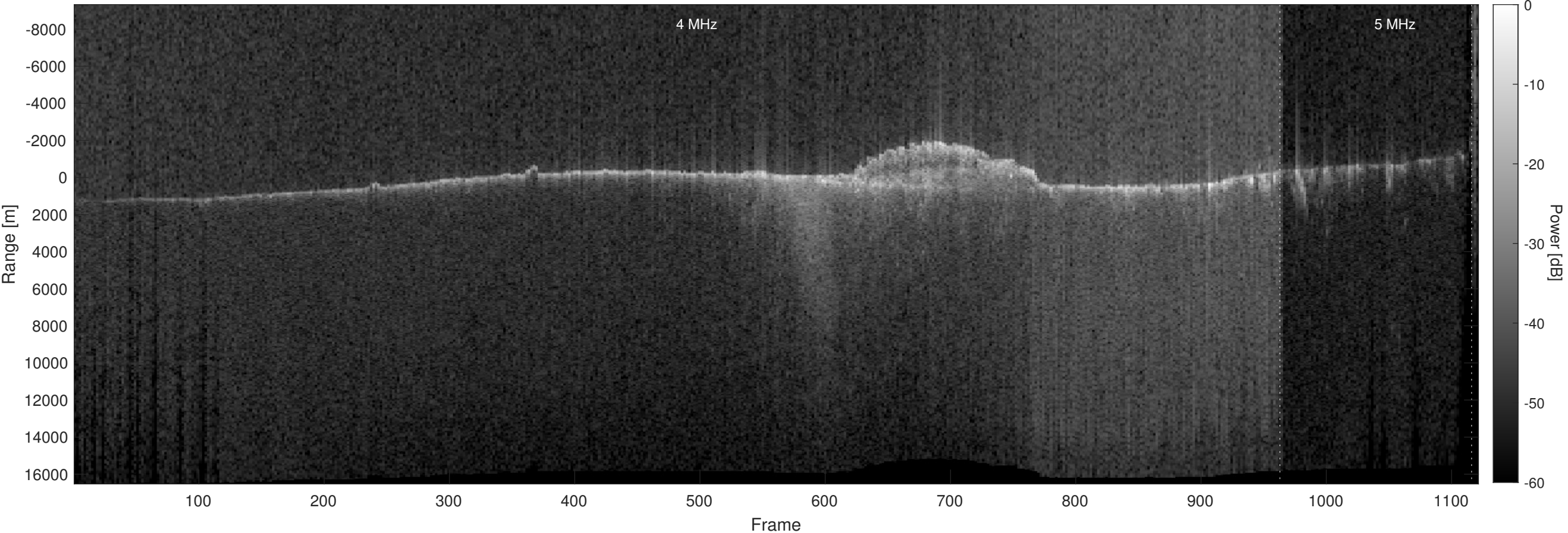
Orbit 14035, Optimized, No Window, Depth-Corrected, Channel 2
