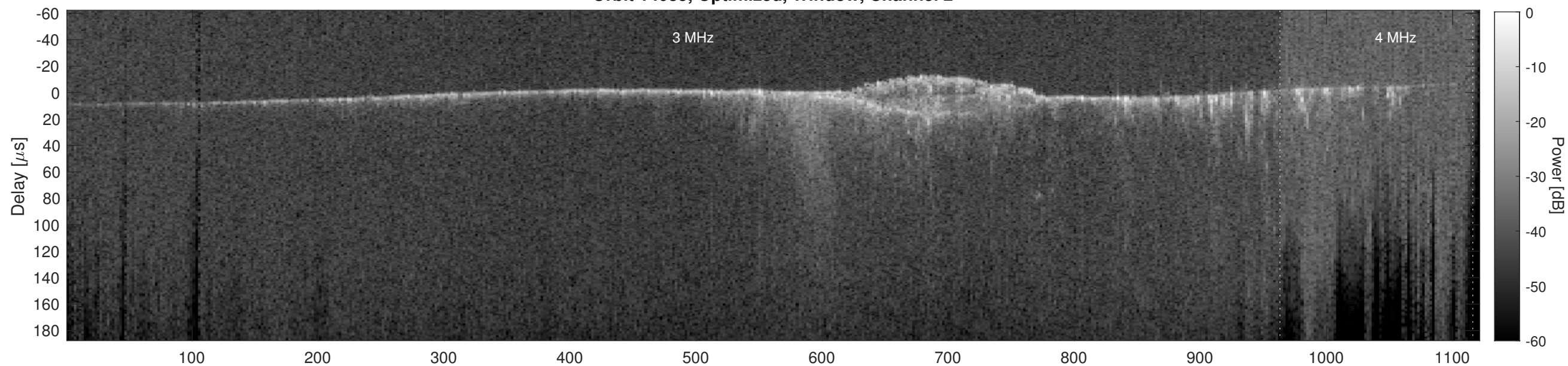
Orbit 14035, Cluttergram
