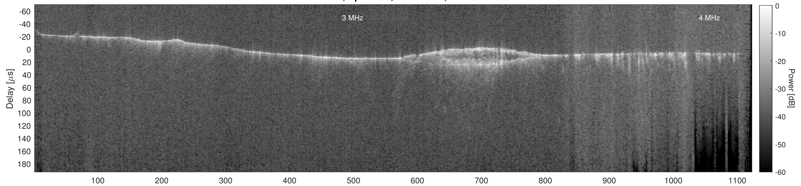
Orbit 14037, Cluttergram
