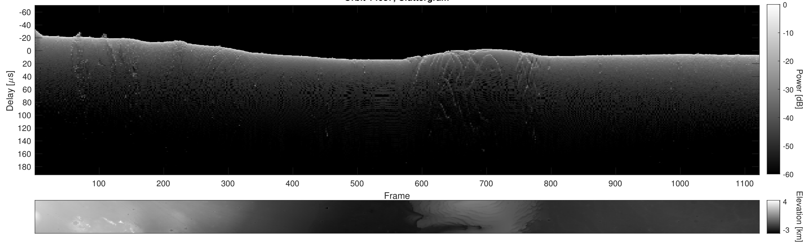
Orbit 14037, Cluttergram
