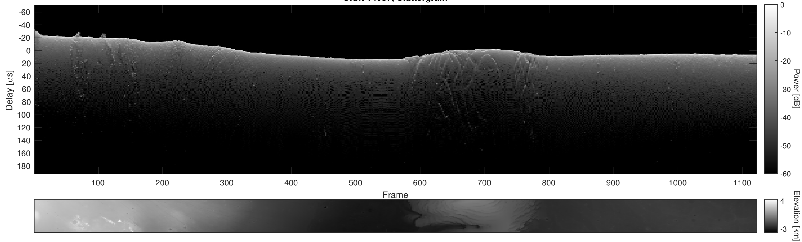
Orbit 14037, Cluttergram
