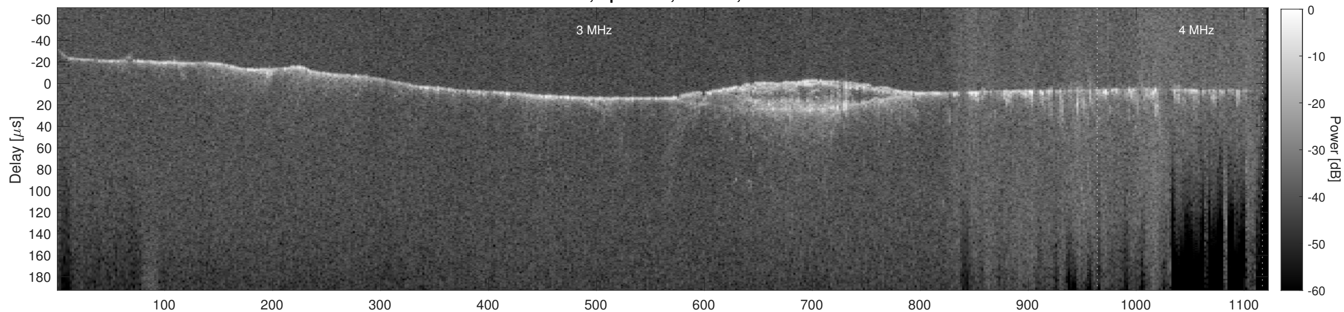
Orbit 14037, Cluttergram
