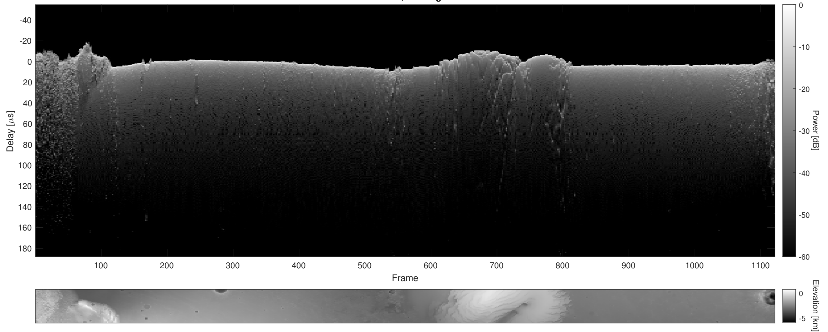
Orbit 14041, Cluttergram
