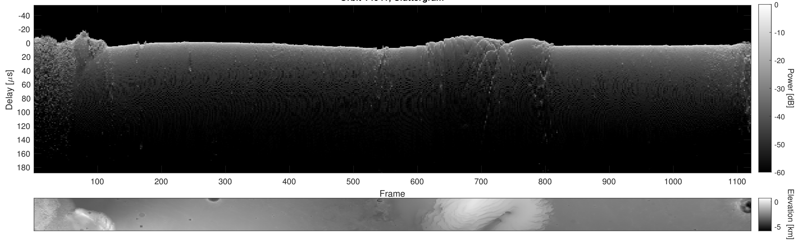
Orbit 14041, Cluttergram
