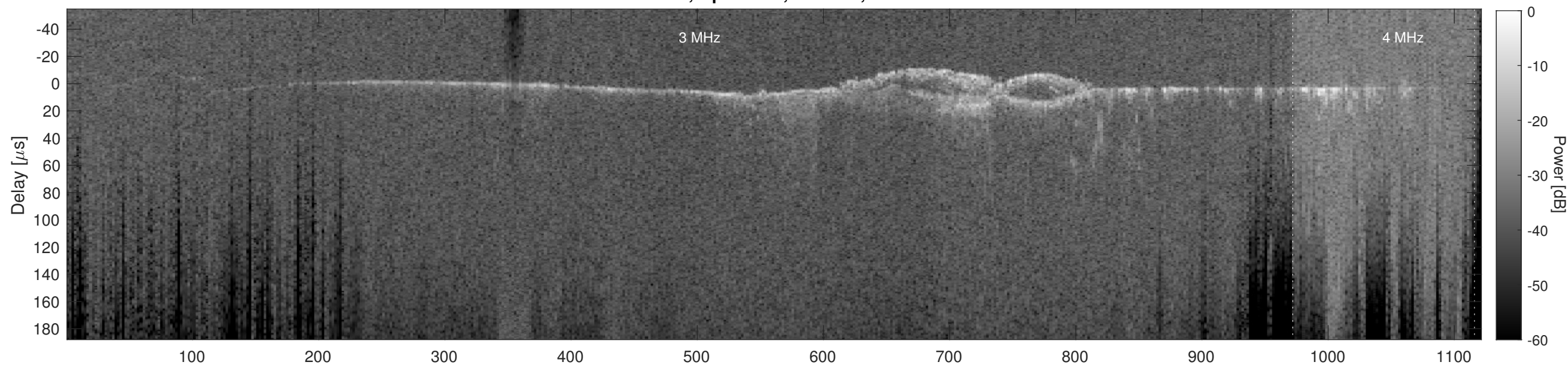
Orbit 14041, Cluttergram
