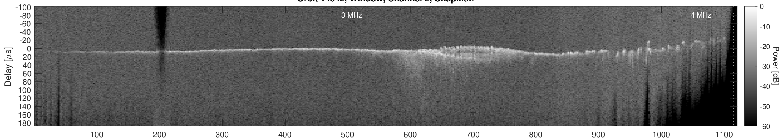
Orbit 14042, Window, Channel 2, Optimized
