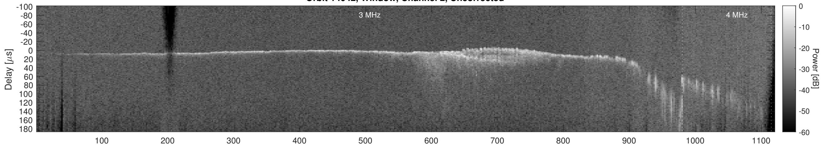
Orbit 14042, Window, Channel 2, Chapman
