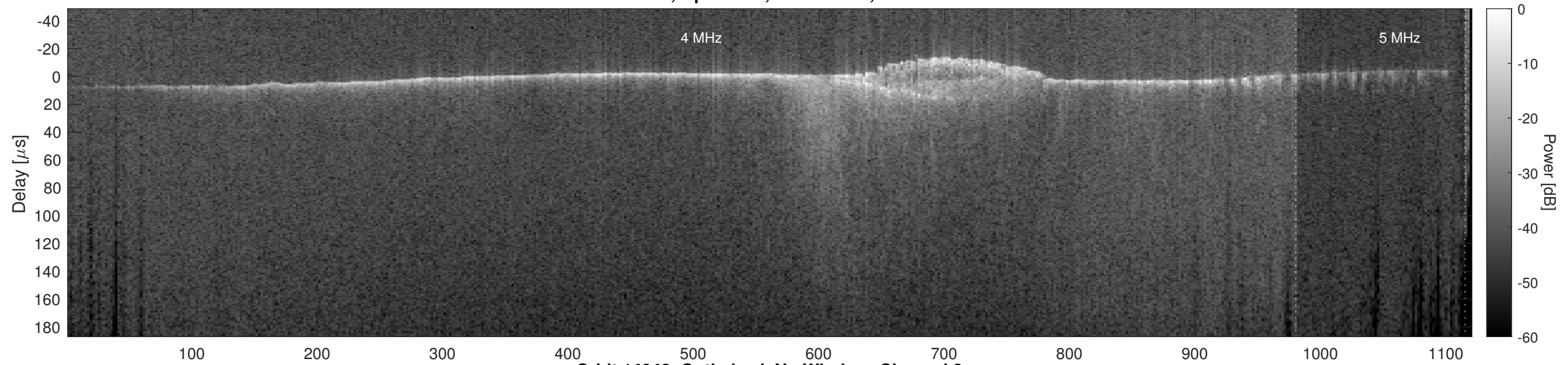
Orbit 14042, Optimized, No Window, Channel 2
