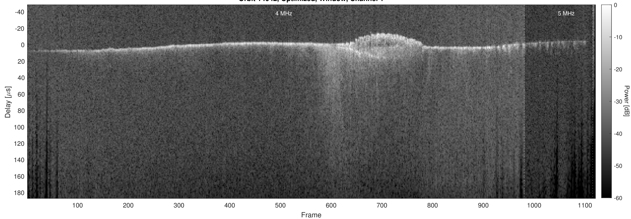
Orbit 14042, Optimized, Window, Channel 2
