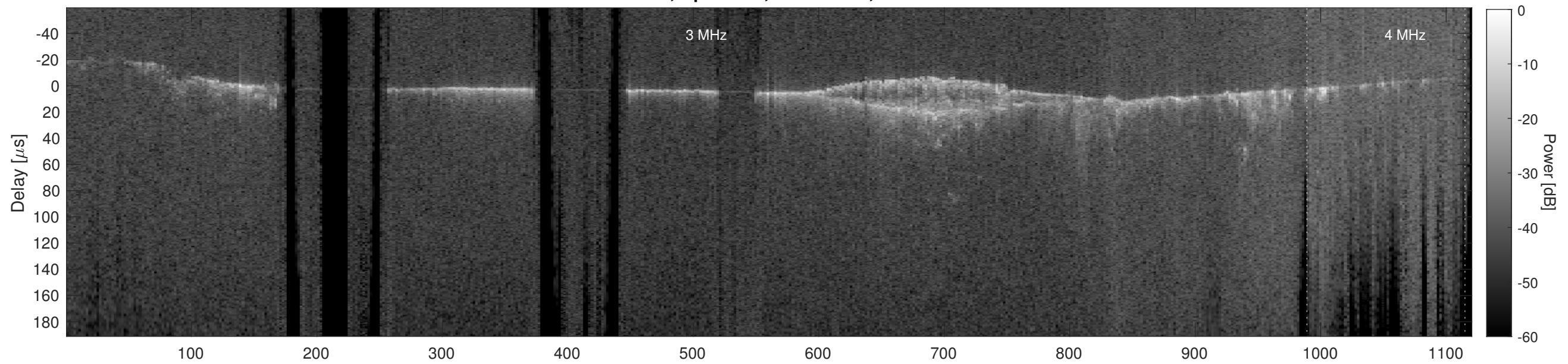
Orbit 14046, Cluttergram
