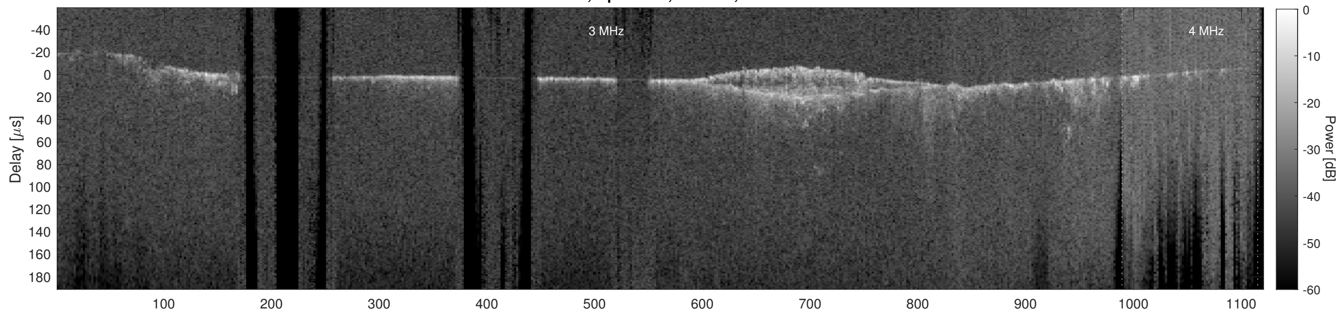
Orbit 14046, Cluttergram
