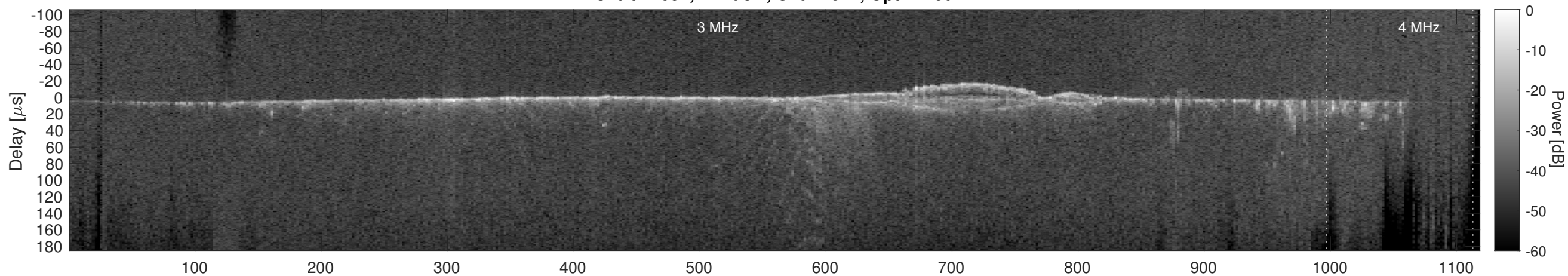
Orbit 14052, Cluttergram
