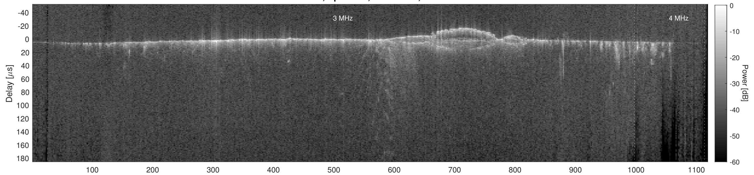
Orbit 14052, Cluttergram
