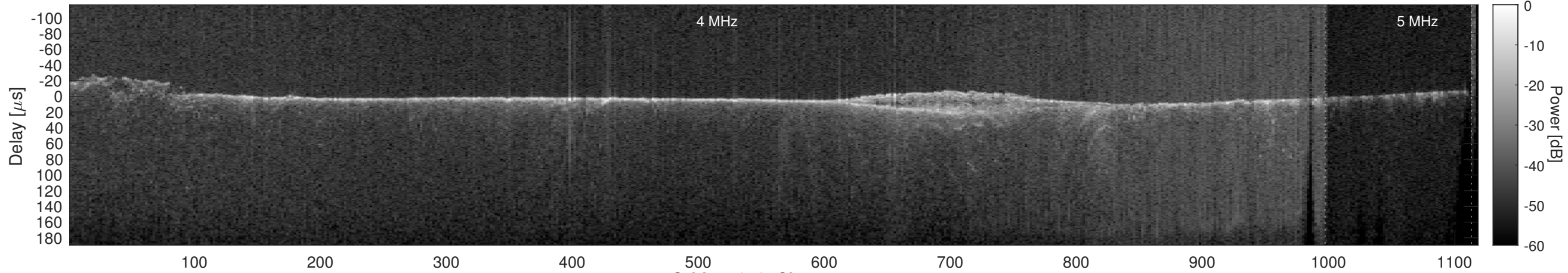
Orbit 14053, Cluttergram
