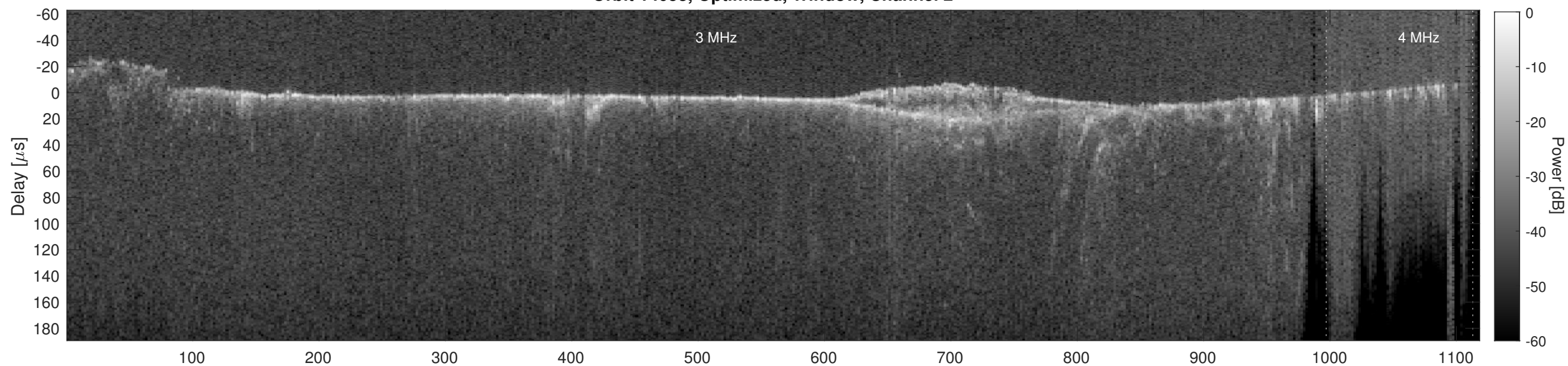
Orbit 14053, Cluttergram
