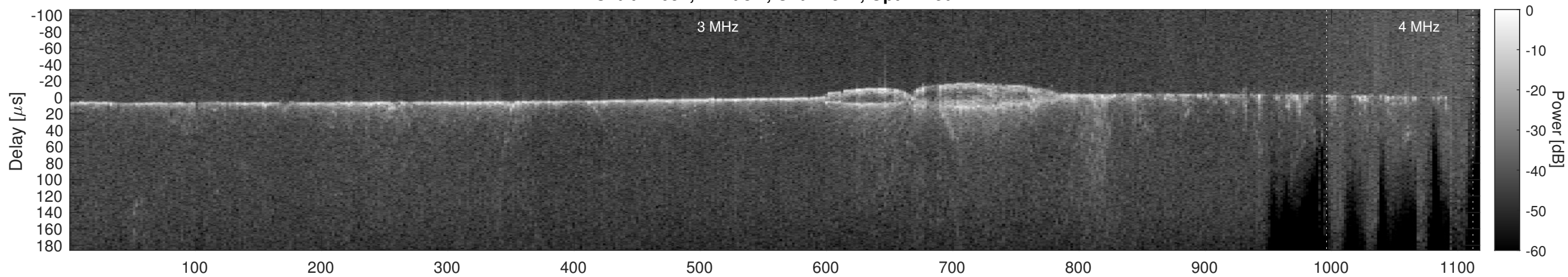
Orbit 14054, Cluttergram
