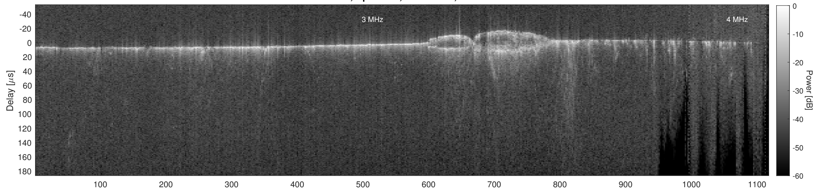
Orbit 14054, Cluttergram
