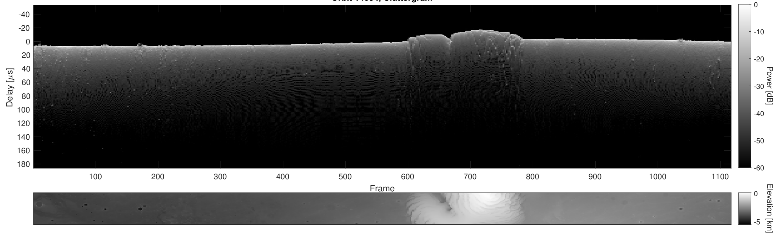
Orbit 14054, Cluttergram
