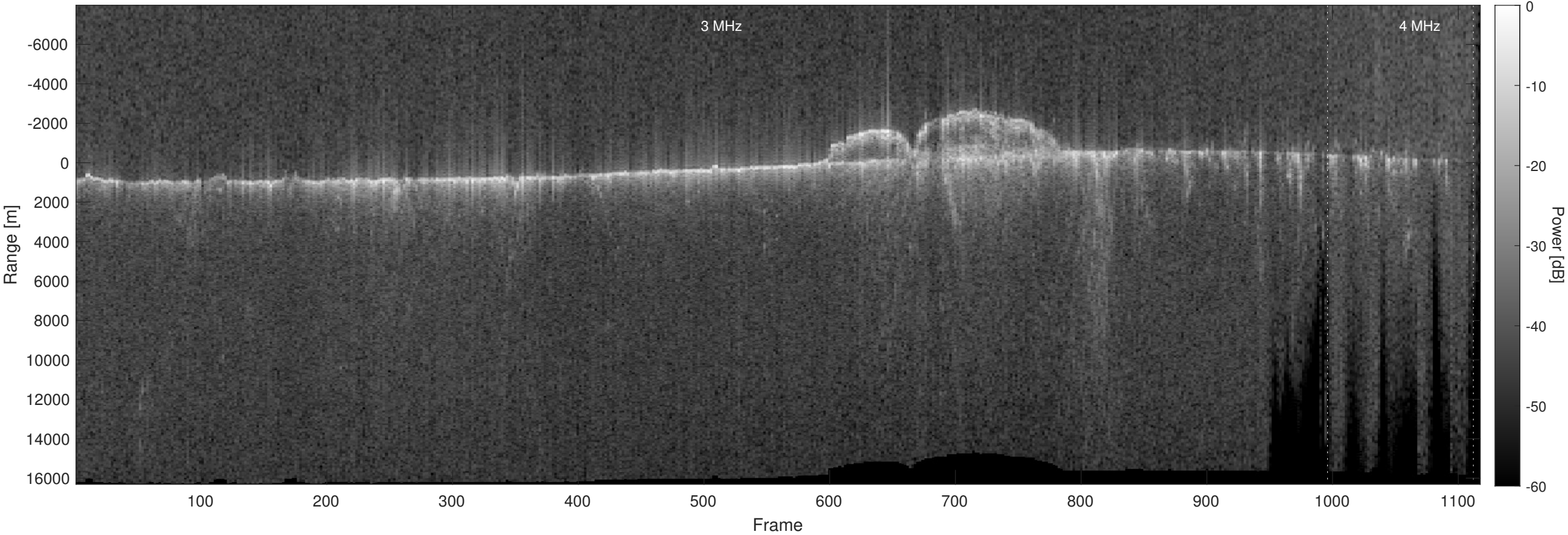
Orbit 14054, Optimized, No Window, Depth-Corrected, Channel 2
