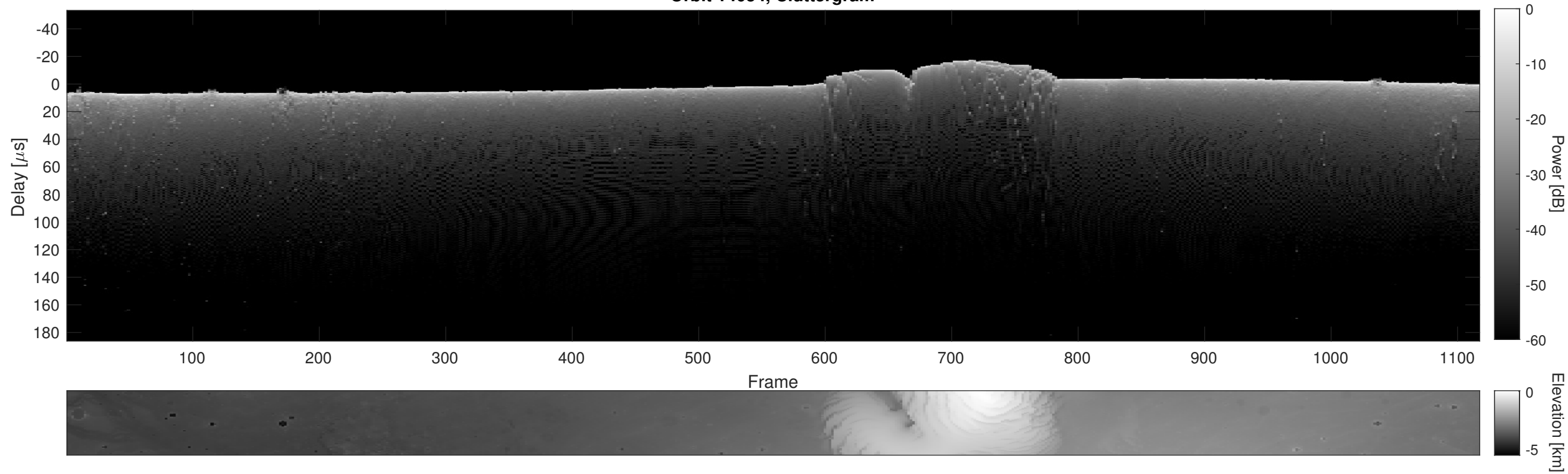
Orbit 14054, Cluttergram
