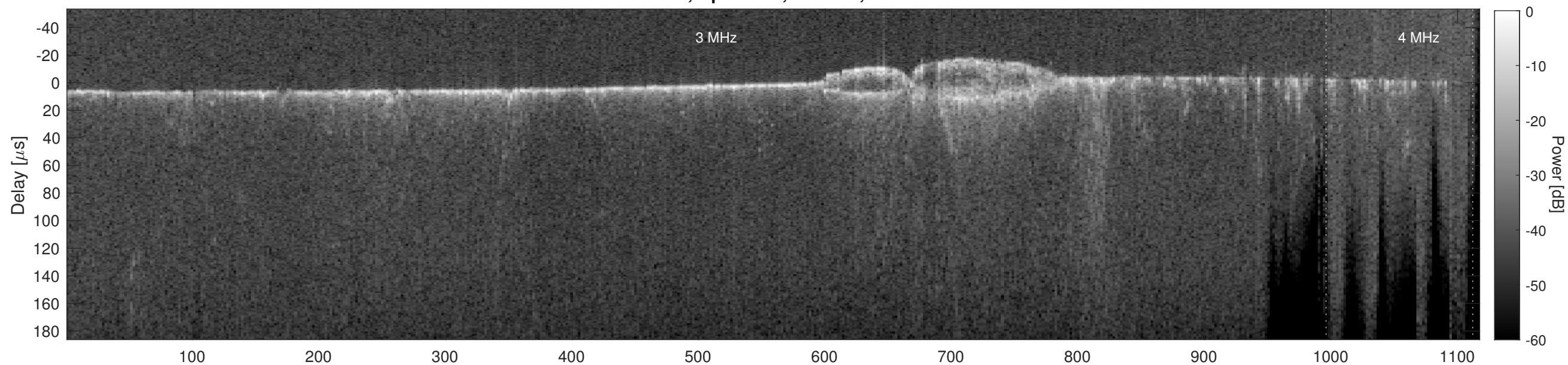
Orbit 14054, Cluttergram
