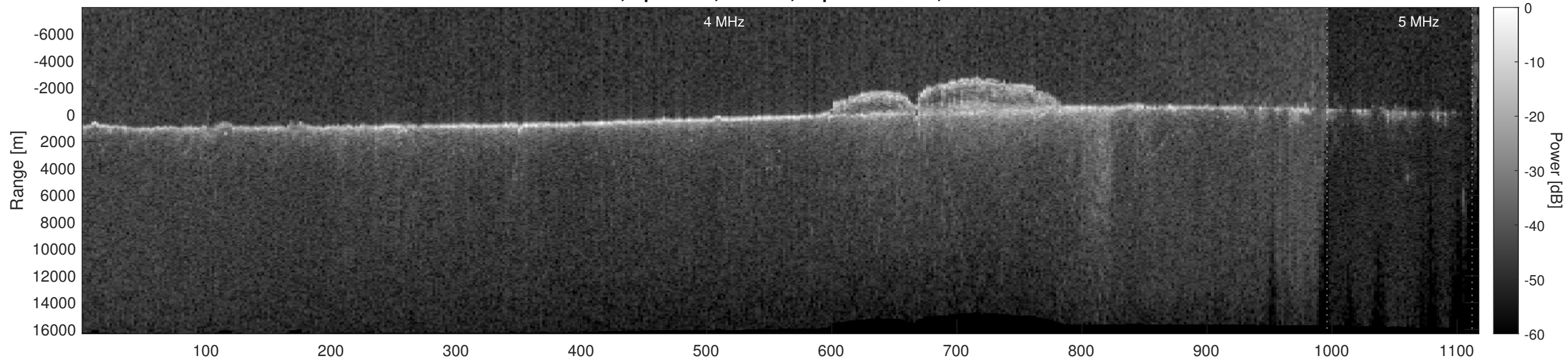
Orbit 14054, Optimized, Window, Depth-Corrected, Channel 2
