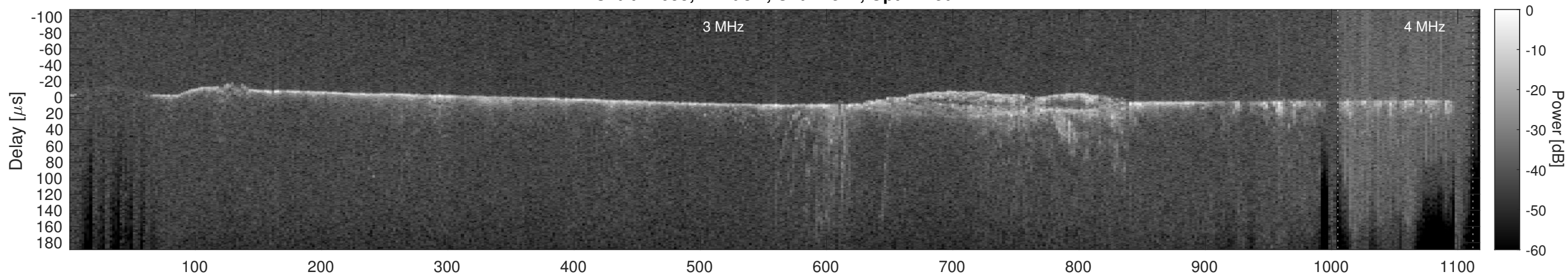
Orbit 14055, Cluttergram
