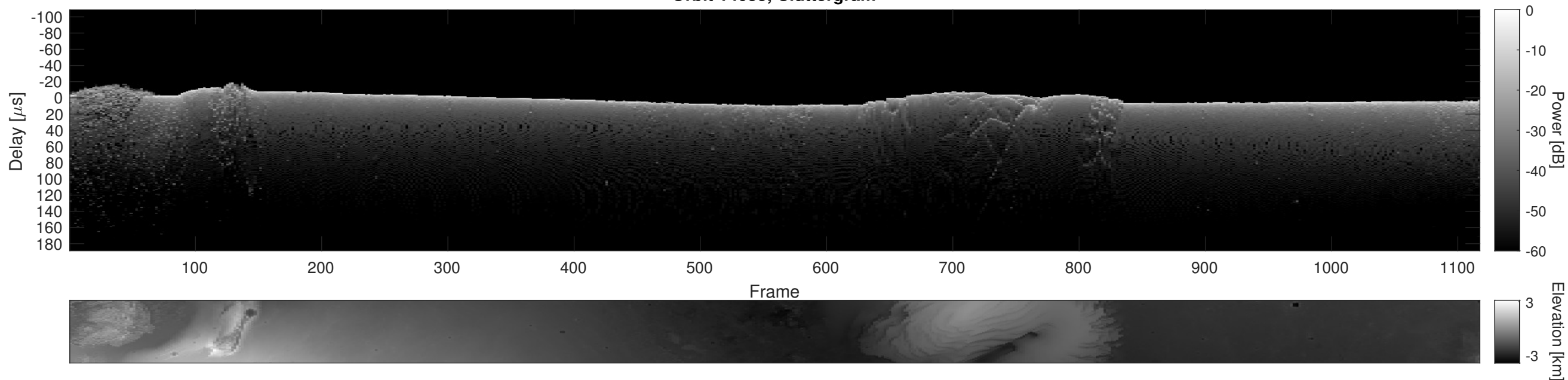
Orbit 14055, Cluttergram
