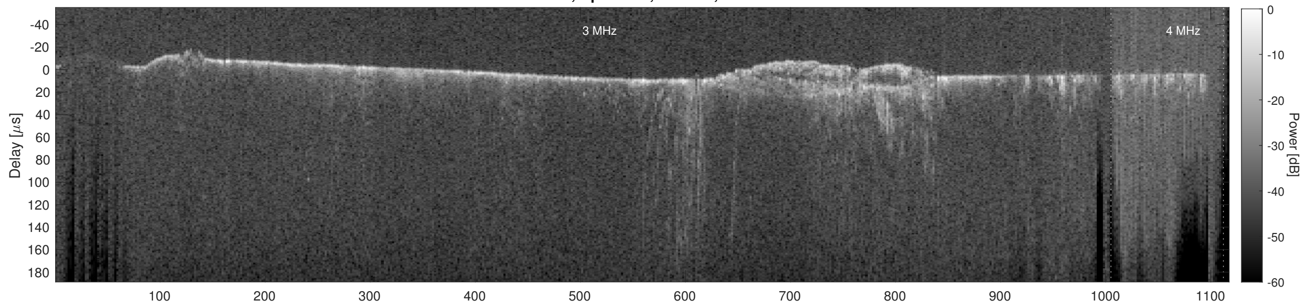
Orbit 14055, Cluttergram
