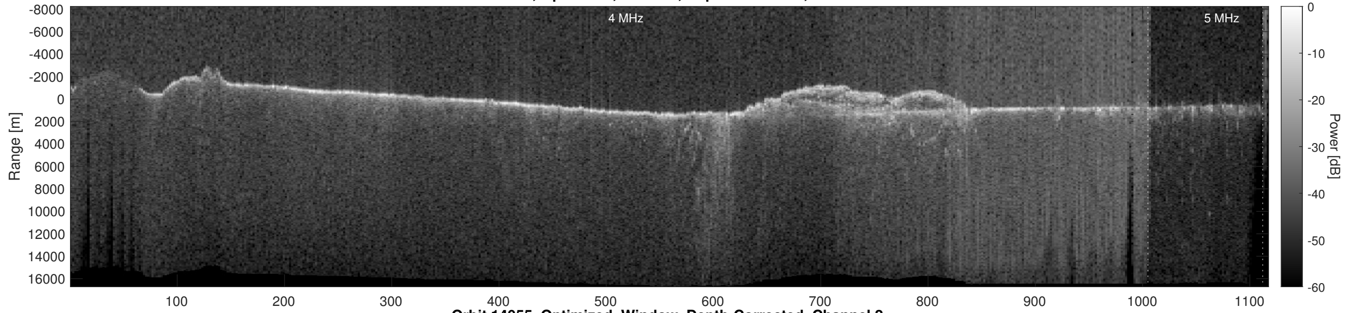
Orbit 14055, Optimized, Window, Depth-Corrected, Channel 2
