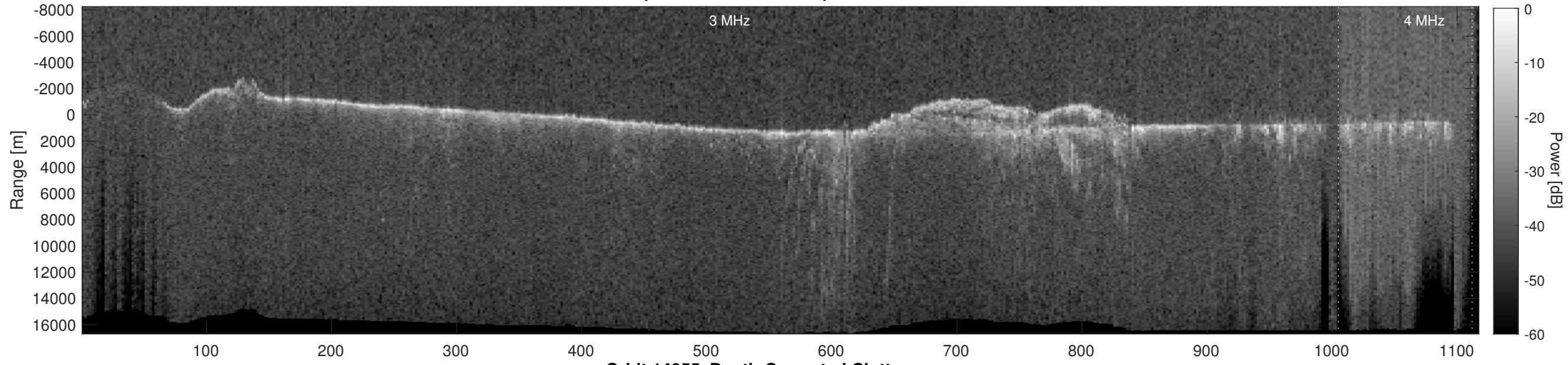
Orbit 14055, Depth-Corrected Cluttergram
