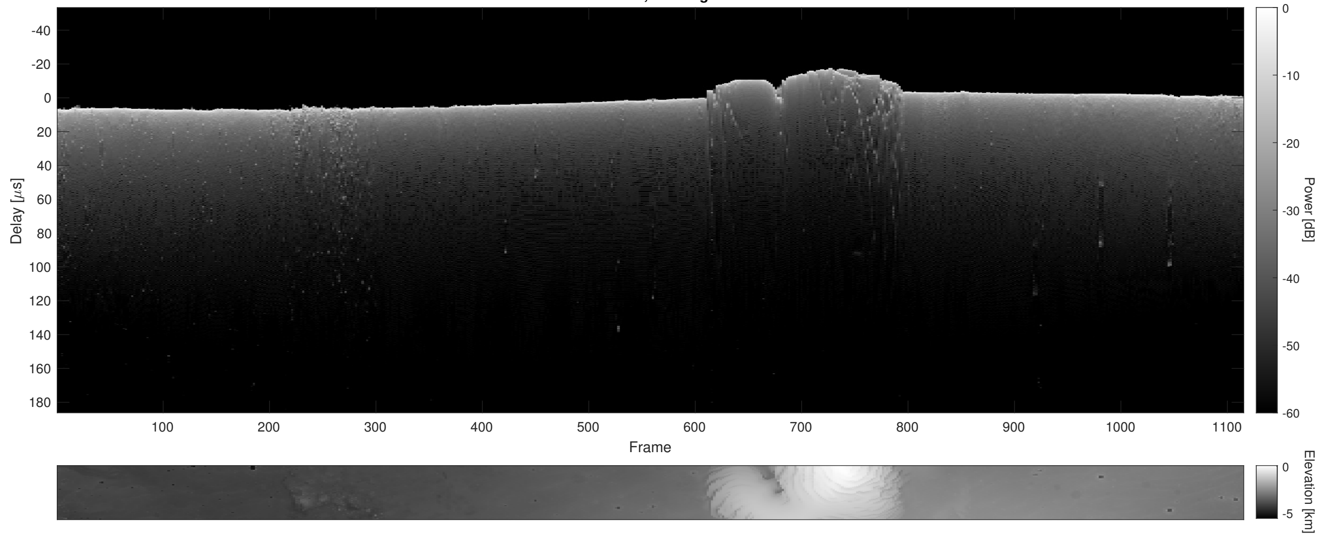
Orbit 14061, Cluttergram
