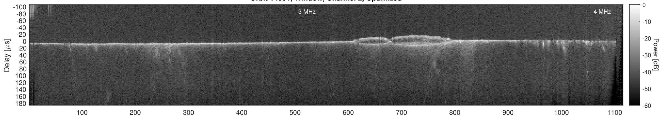
Orbit 14061, Cluttergram
