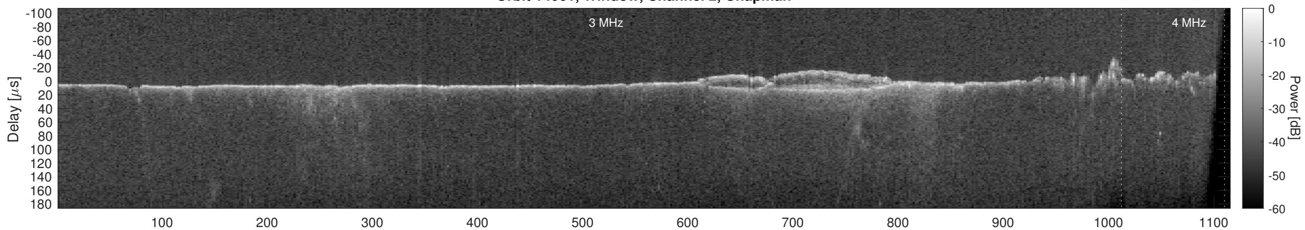
Orbit 14061, Window, Channel 2, Optimized
