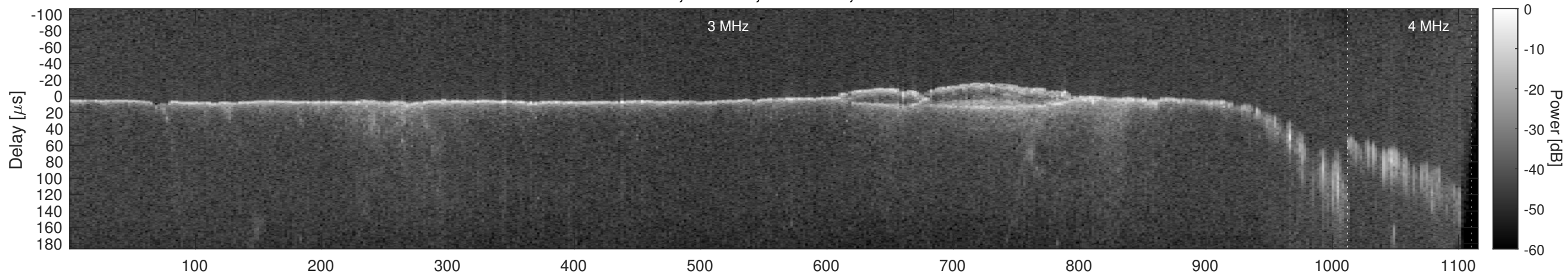
Orbit 14061, Window, Channel 2, Chapman
