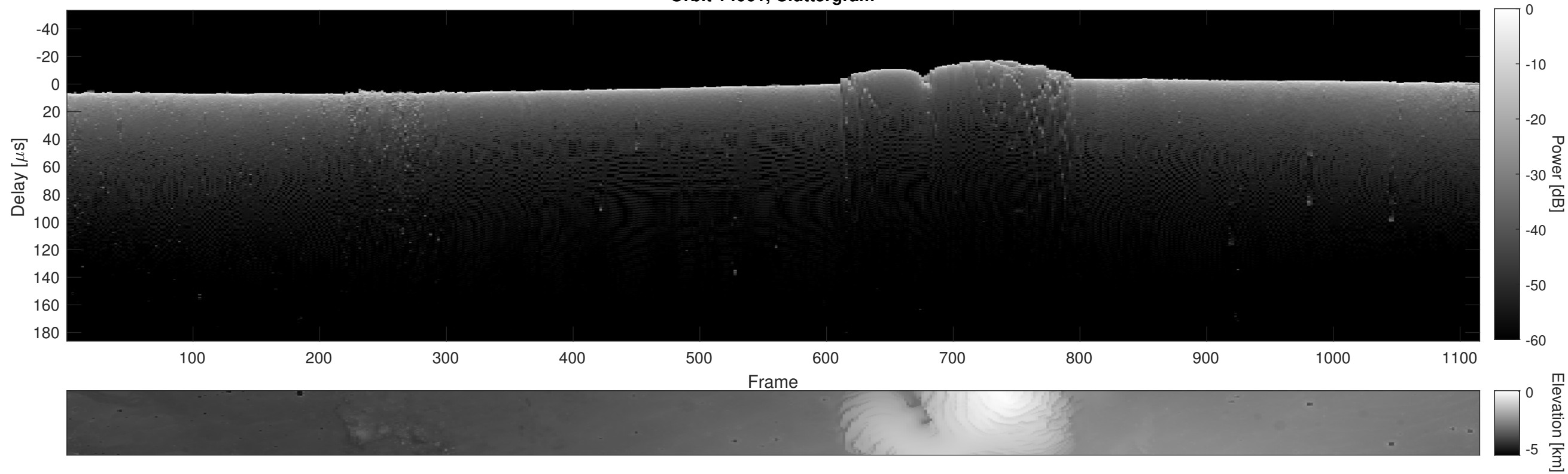
Orbit 14061, Cluttergram
