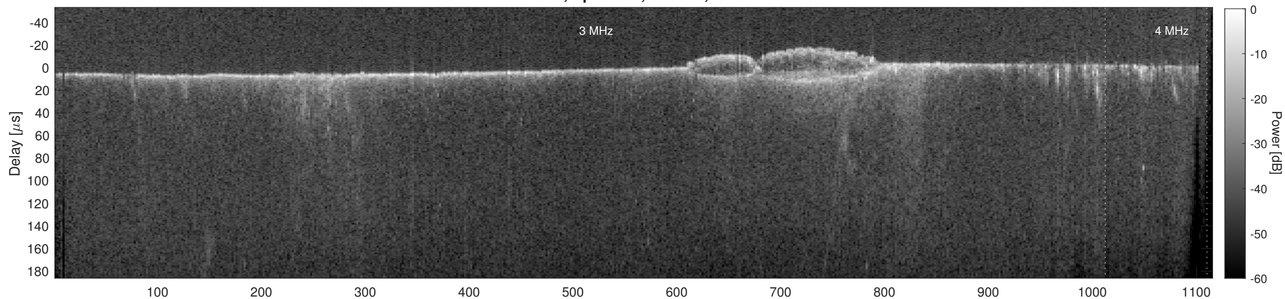
Orbit 14061, Cluttergram
