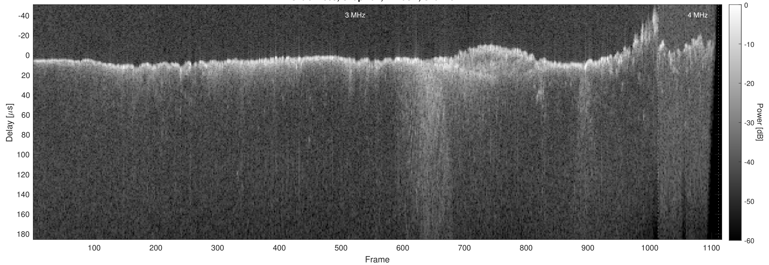
Orbit 14063, Chapman, Window, Channel 2
