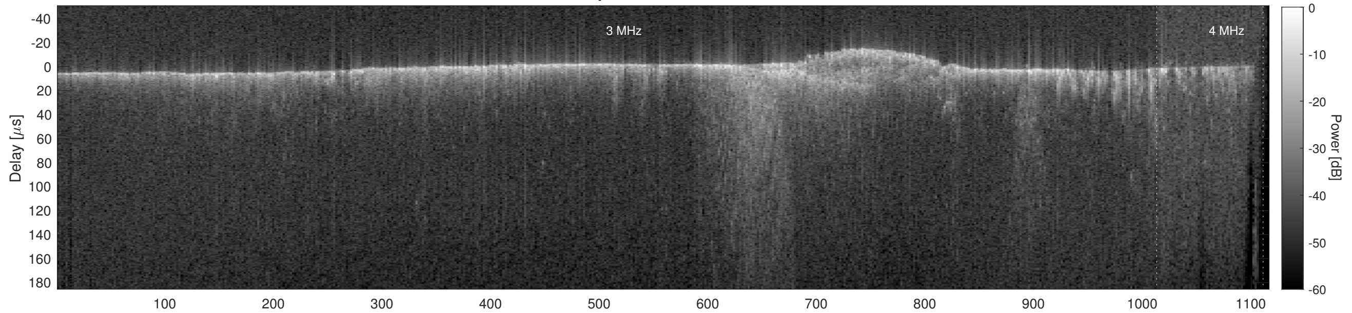
Orbit 14063, Cluttergram
