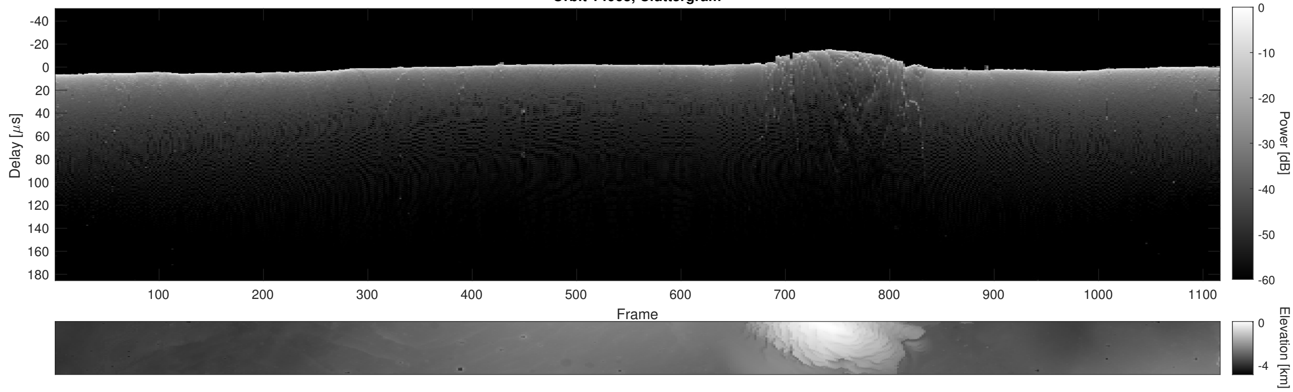
Orbit 14063, Cluttergram
