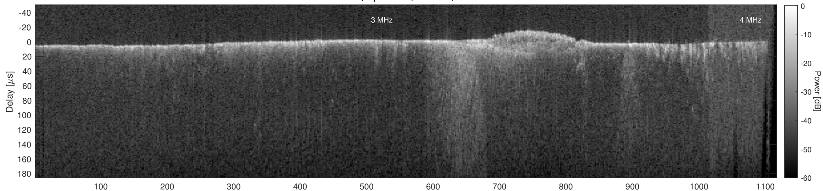
Orbit 14063, Cluttergram
