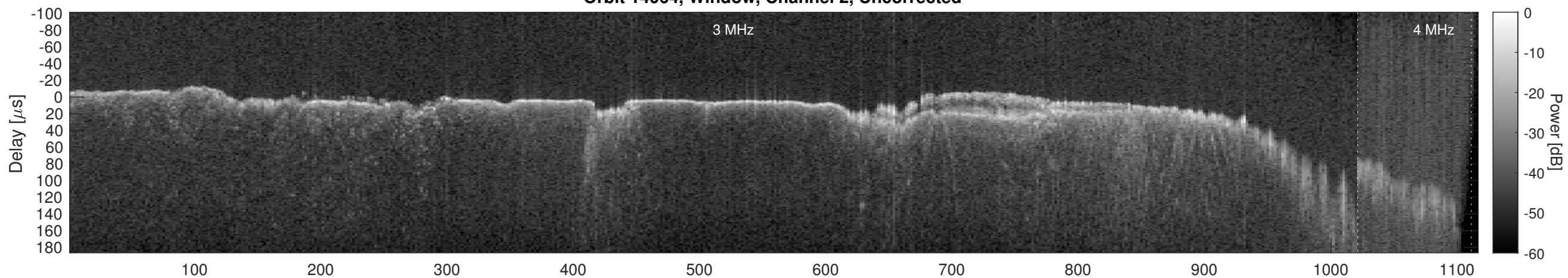
Orbit 14064, Window, Channel 2, Chapman
