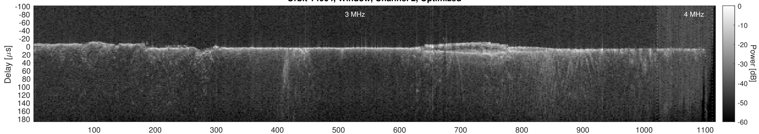
Orbit 14064, Cluttergram
