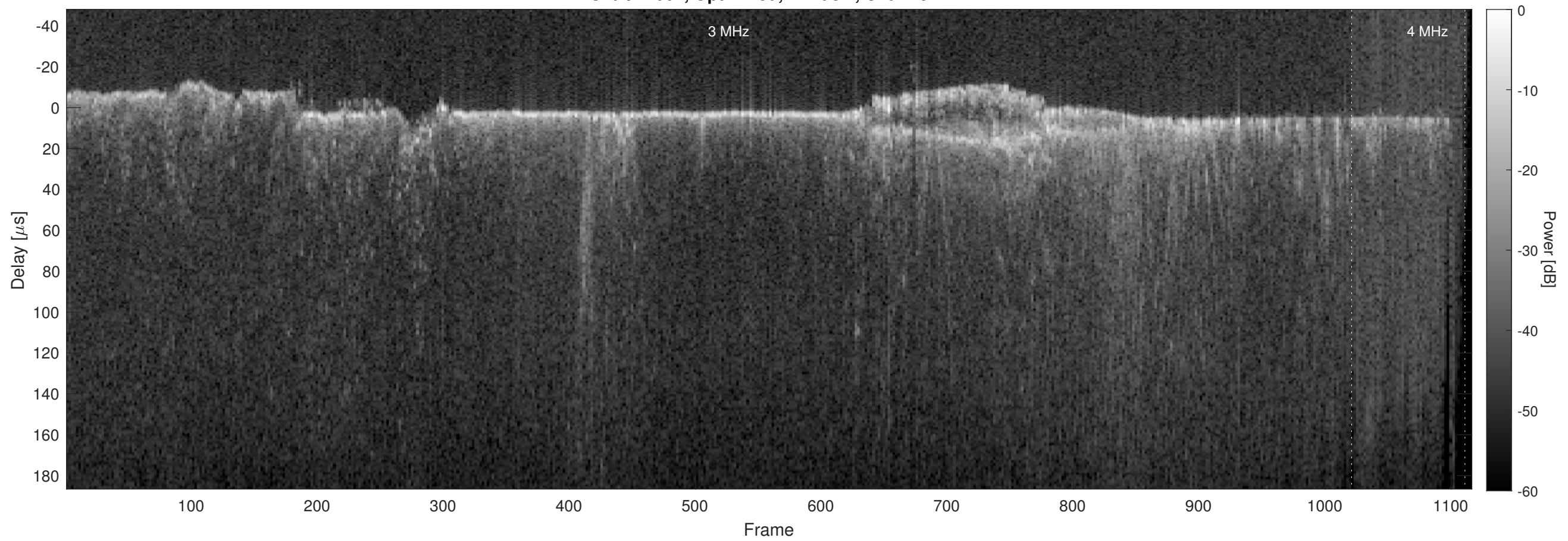
Orbit 14064, Optimized, Window, Channel 2
