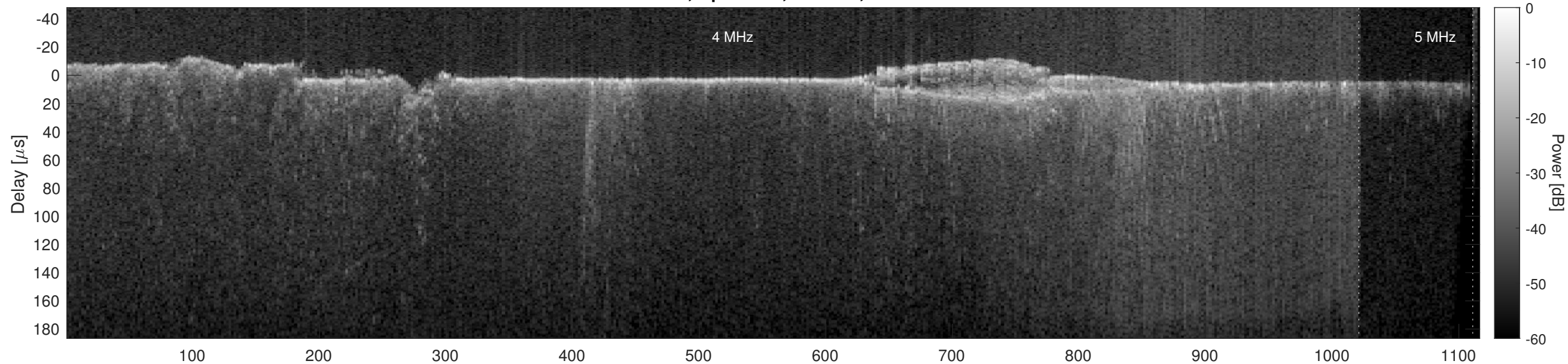
Orbit 14064, Optimized, Window, Channel 2
