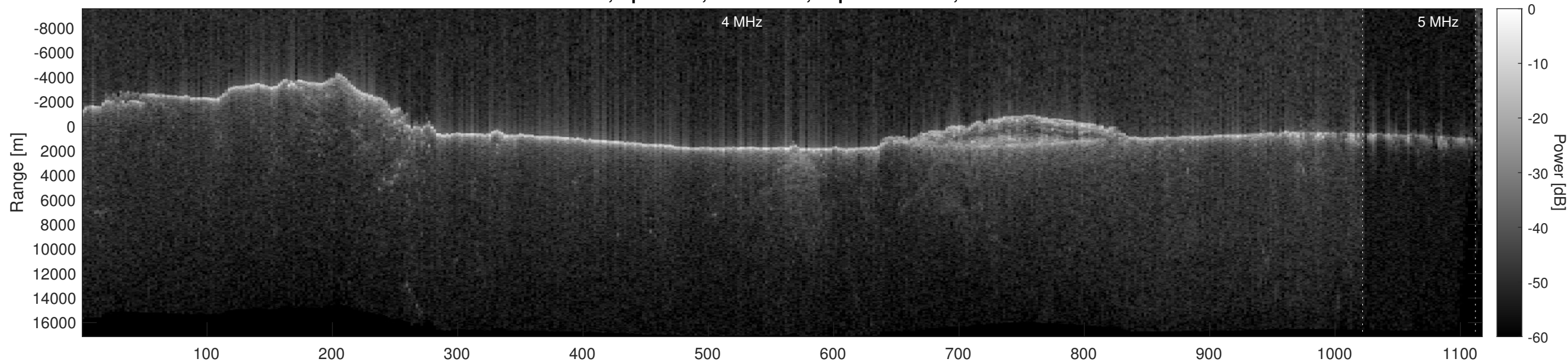
Orbit 14065, Optimized, No Window, Depth-Corrected, Channel 2
