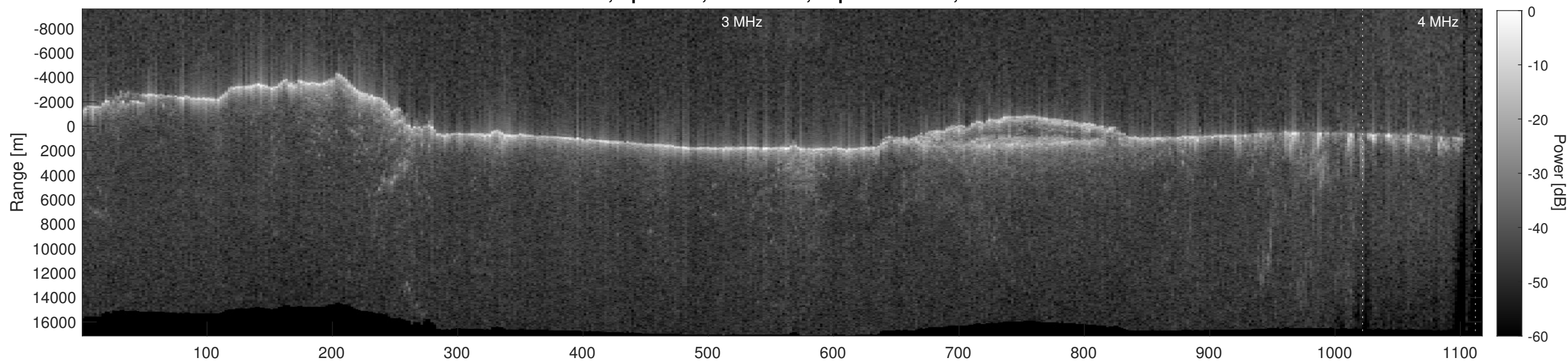
Orbit 14065, Depth-Corrected Cluttergram
