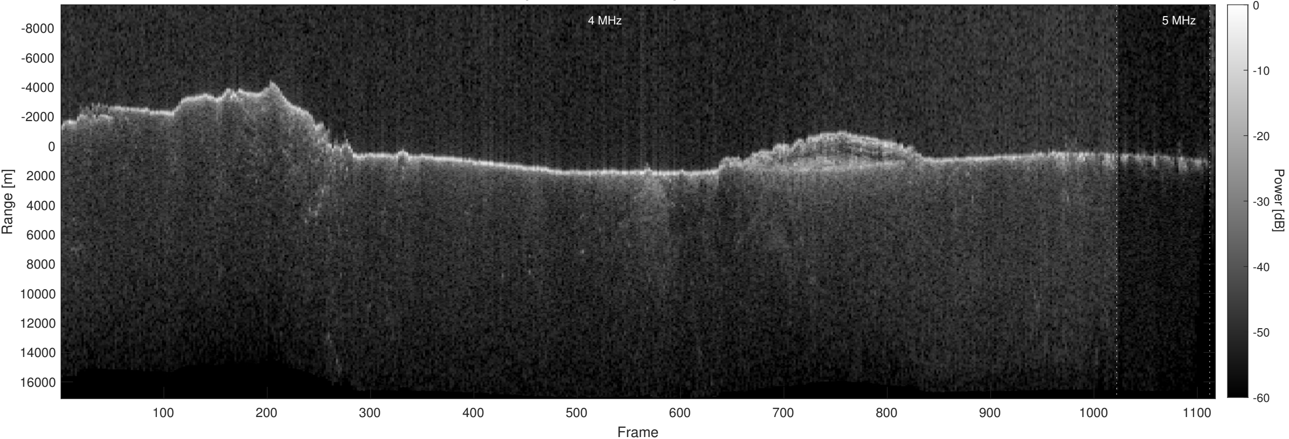
Orbit 14065, Optimized, Window, Depth-Corrected, Channel 2
