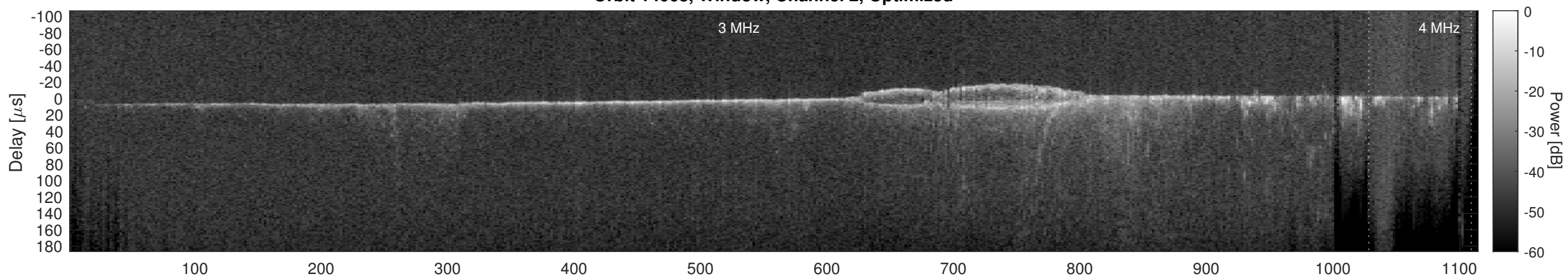
Orbit 14068, Cluttergram
