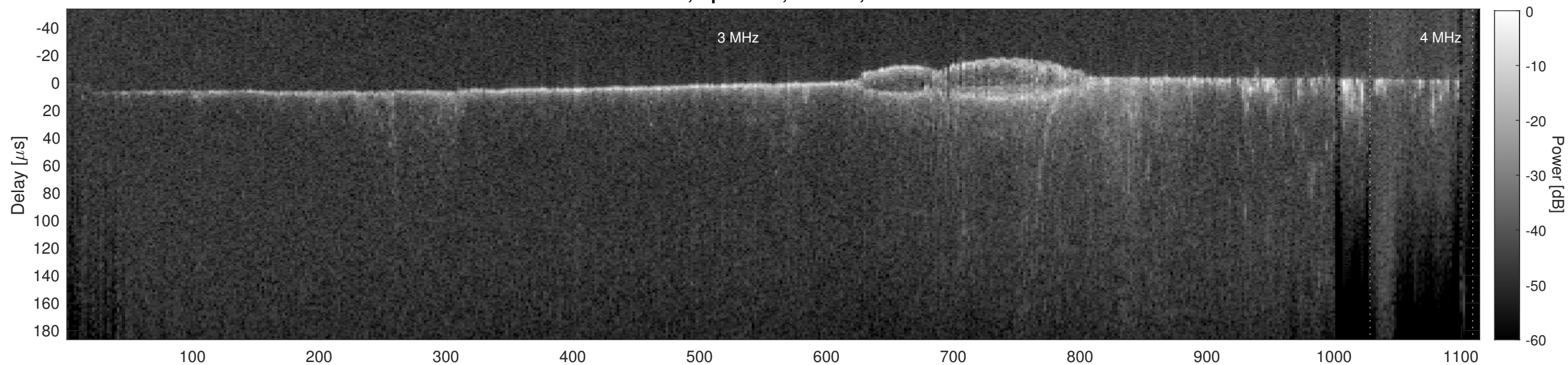
Orbit 14068, Cluttergram
