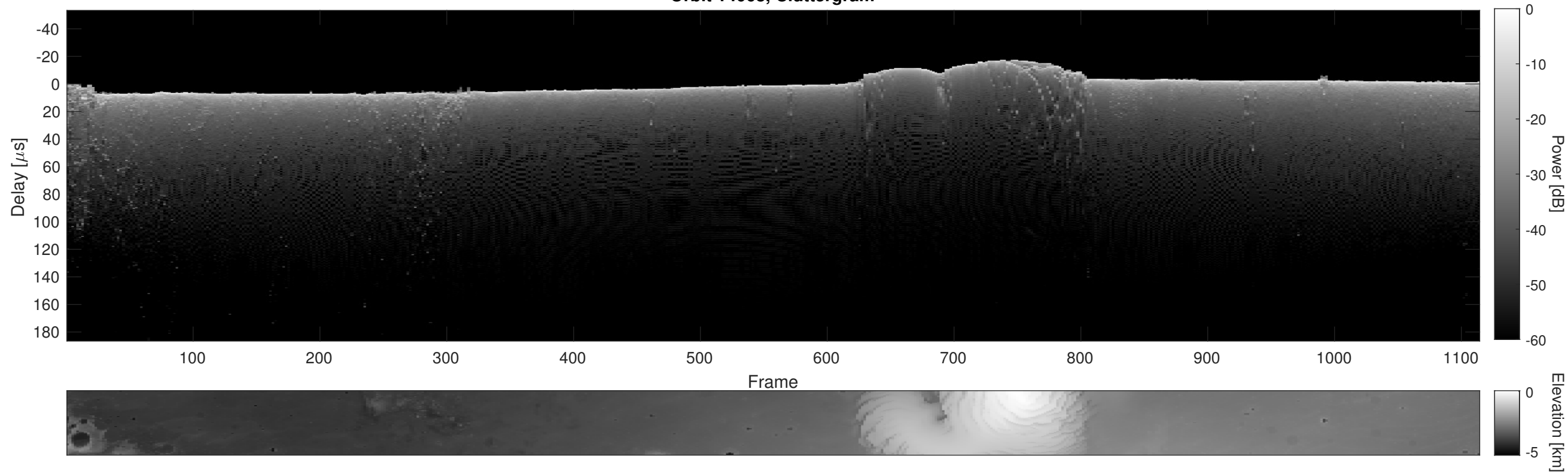
Orbit 14068, Cluttergram
