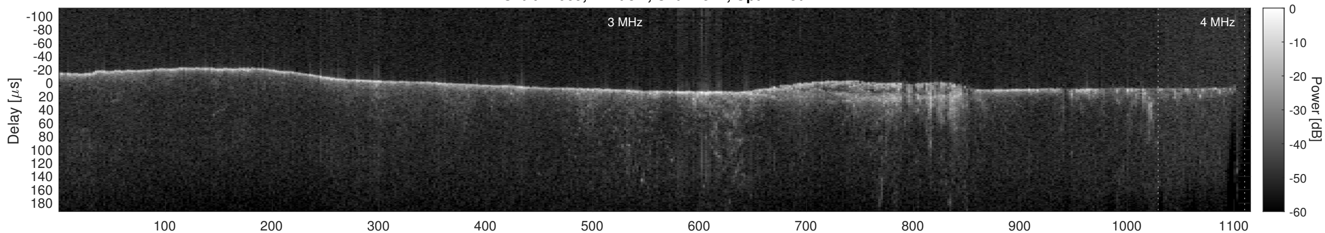
Orbit 14069, Cluttergram
