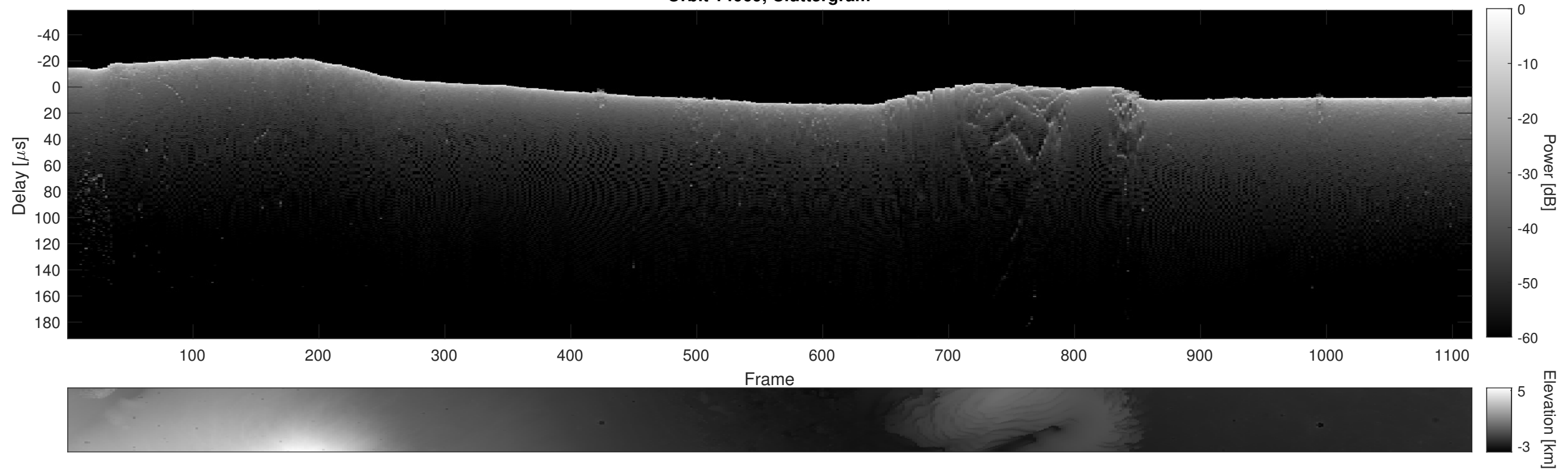
Orbit 14069, Cluttergram
