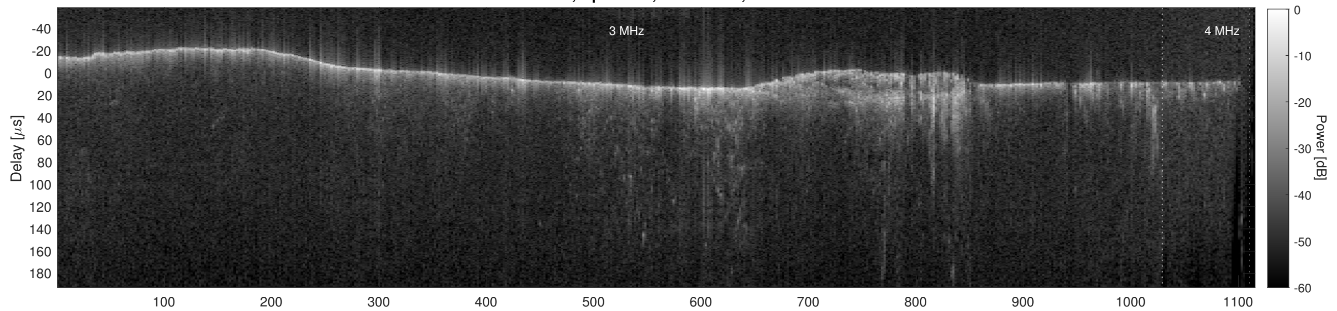
Orbit 14069, Cluttergram
