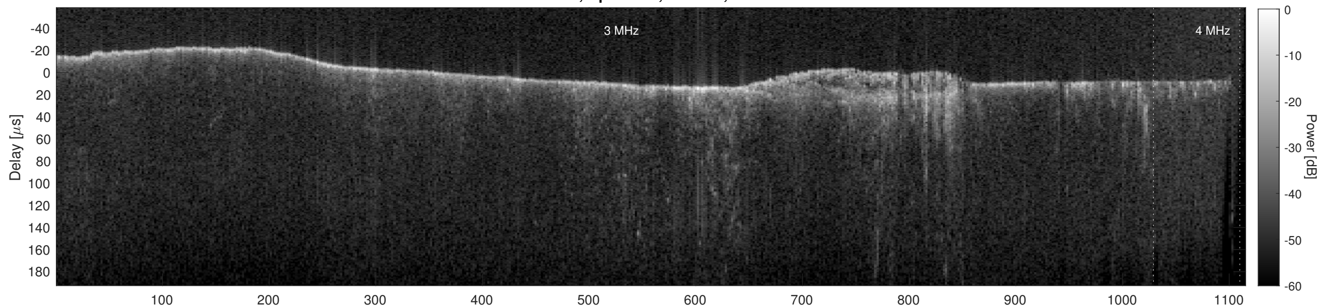
Orbit 14069, Cluttergram
