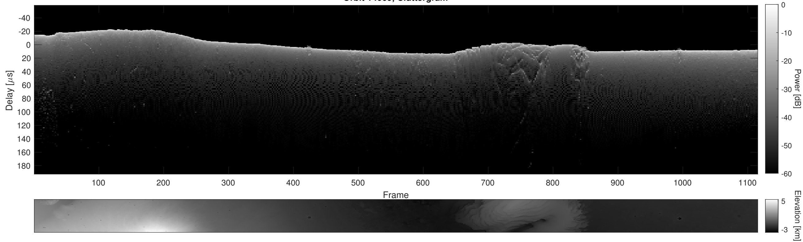
Orbit 14069, Cluttergram
