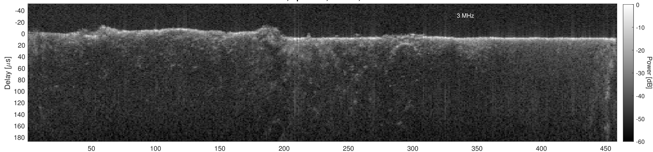
Orbit 14071, Cluttergram
