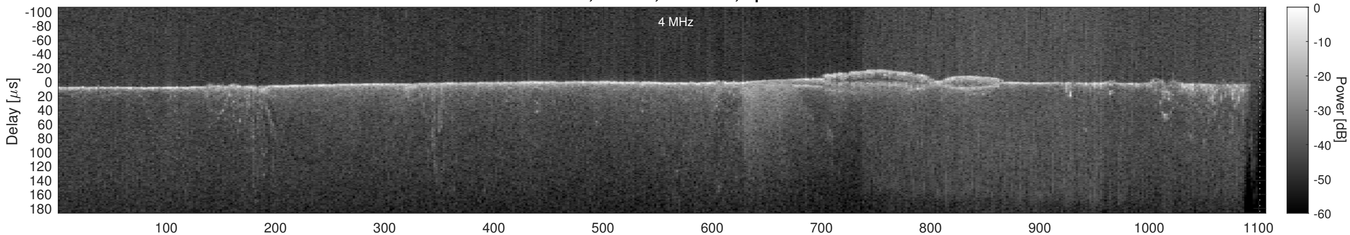
Orbit 14073, Cluttergram
