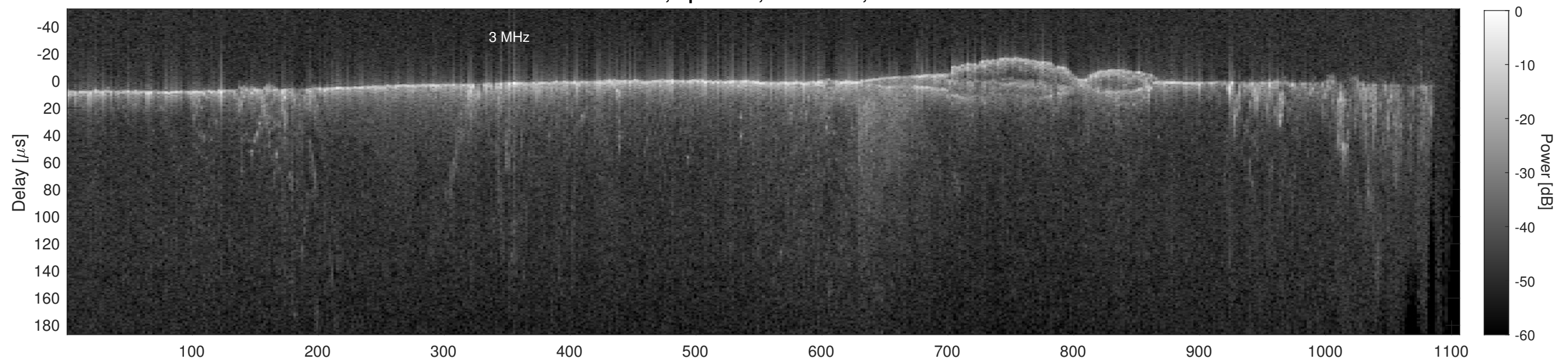
Orbit 14073, Cluttergram
