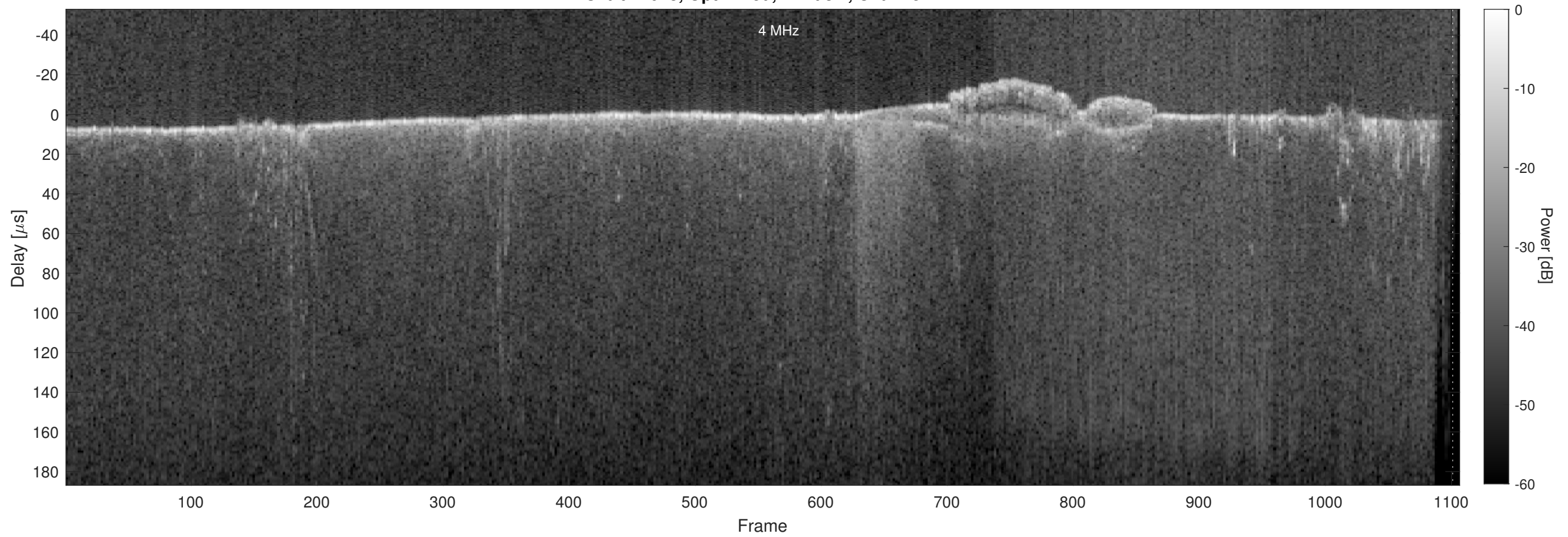
Orbit 14073, Optimized, Window, Channel 2
