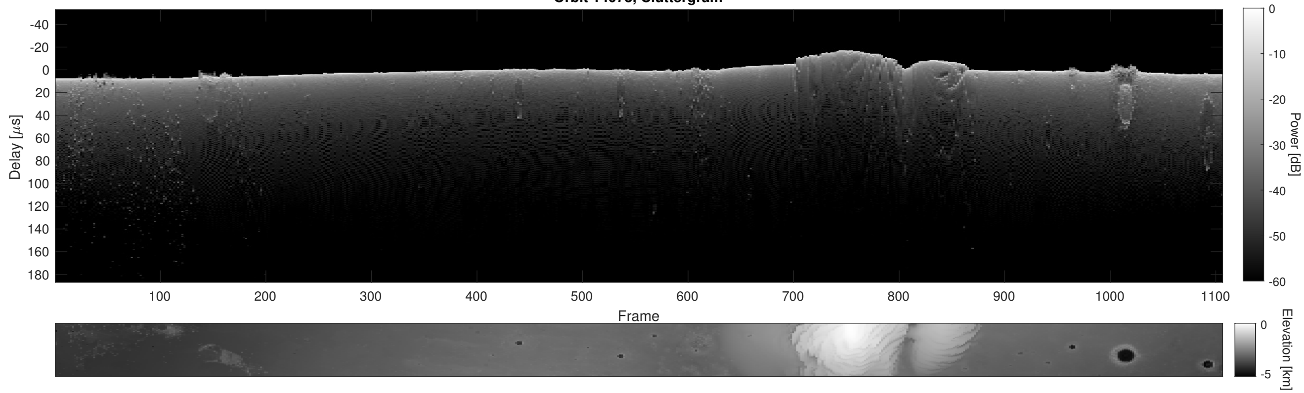
Orbit 14073, Cluttergram
