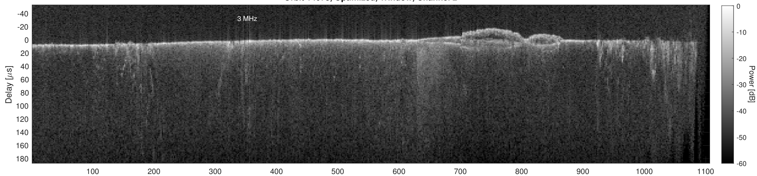
Orbit 14073, Cluttergram
