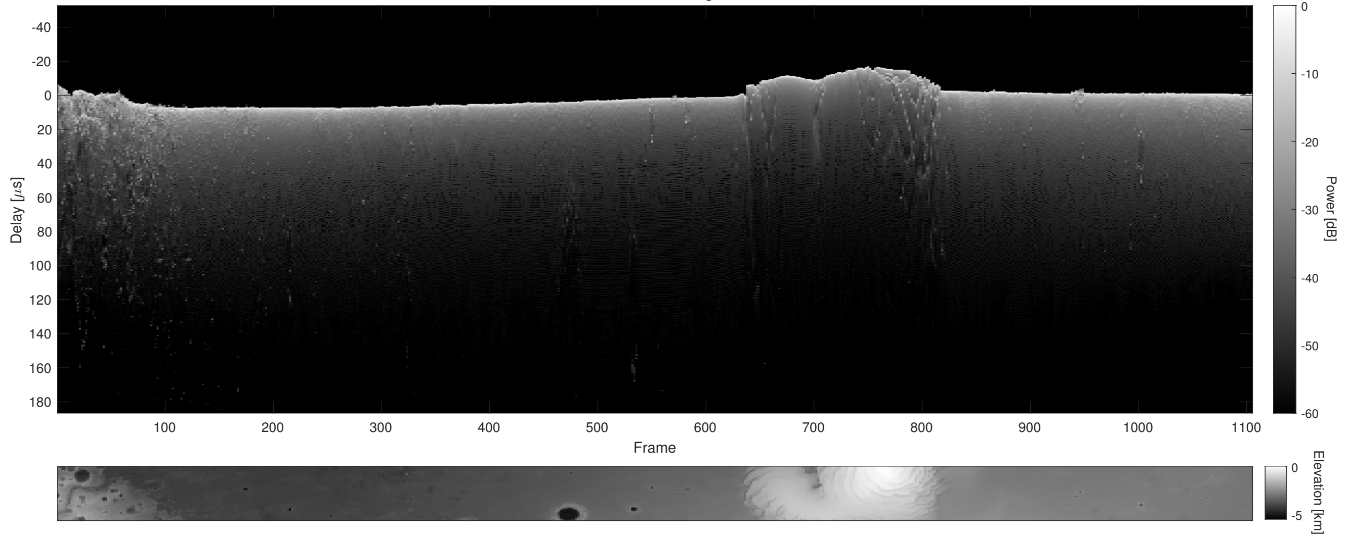
Orbit 14075, Cluttergram
