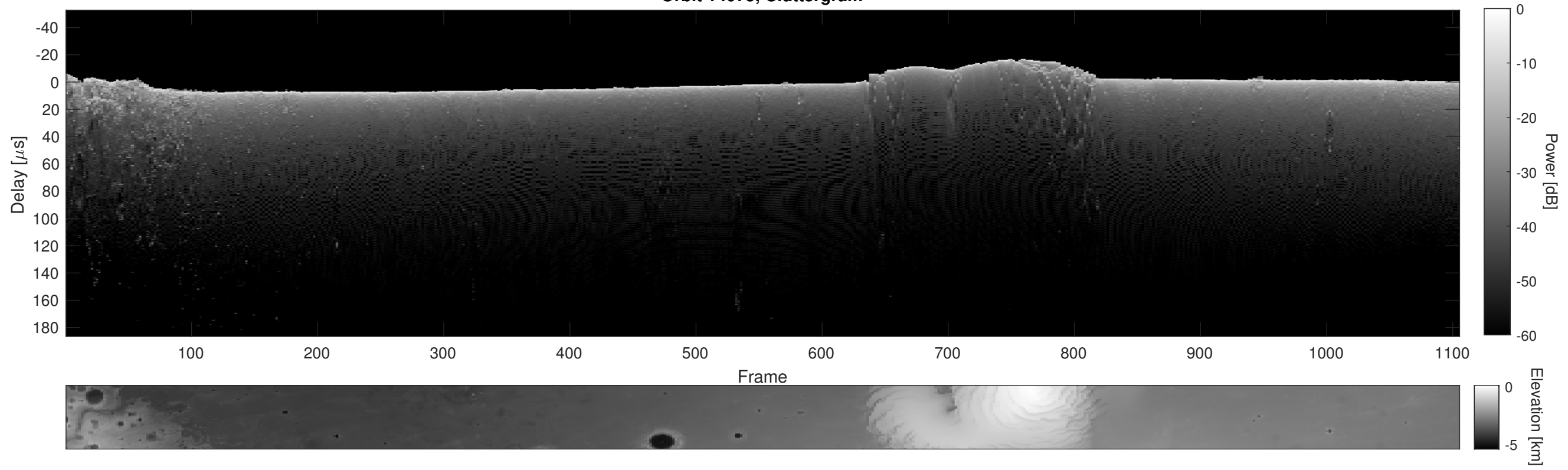
Orbit 14075, Cluttergram
