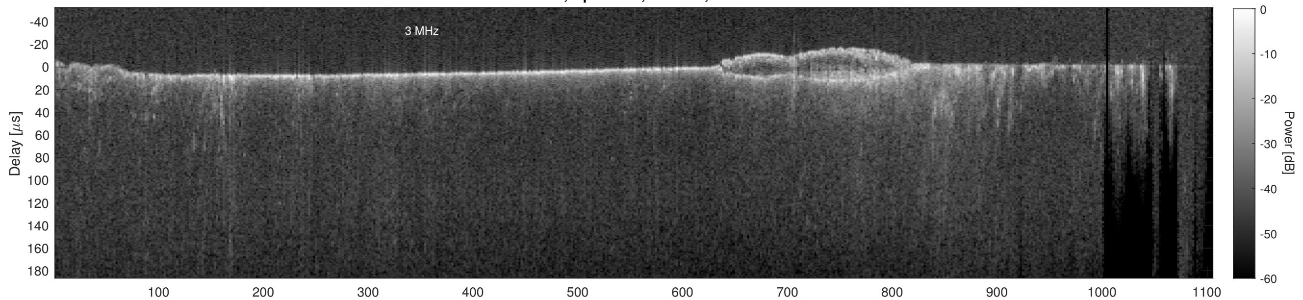
Orbit 14075, Cluttergram
