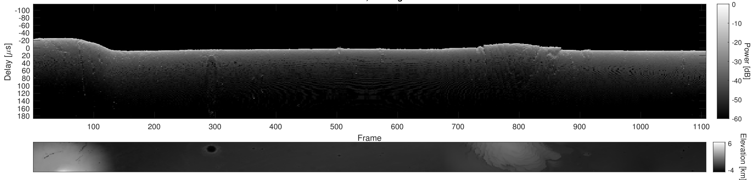
Orbit 14084, Cluttergram
