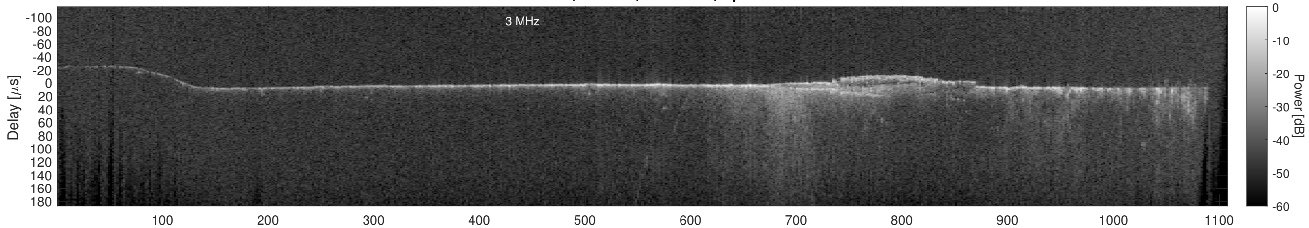
Orbit 14084, Cluttergram
