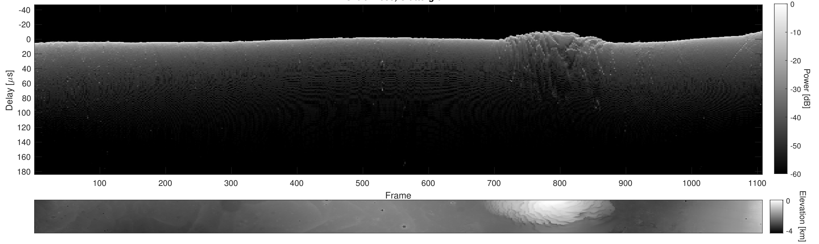
Orbit 14088, Cluttergram
