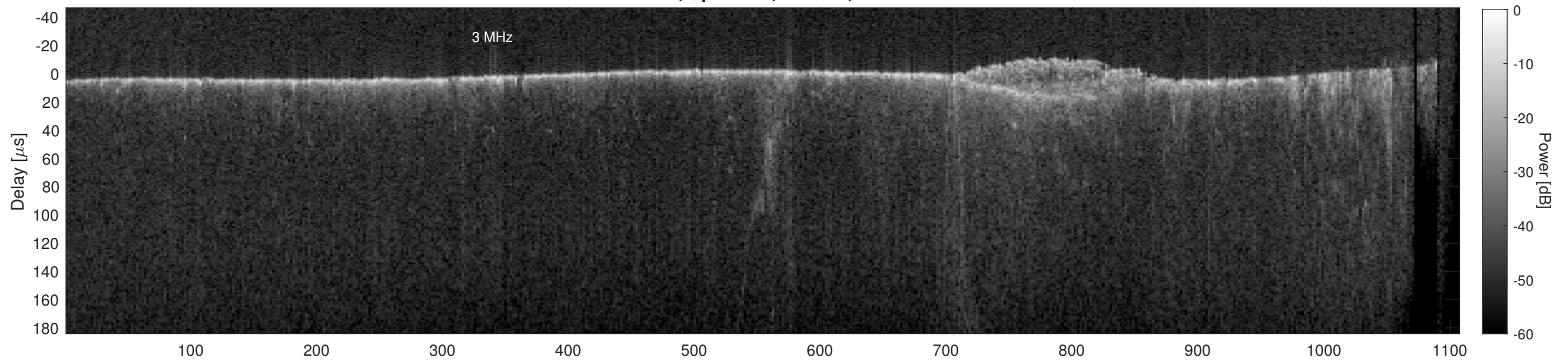
Orbit 14088, Cluttergram
