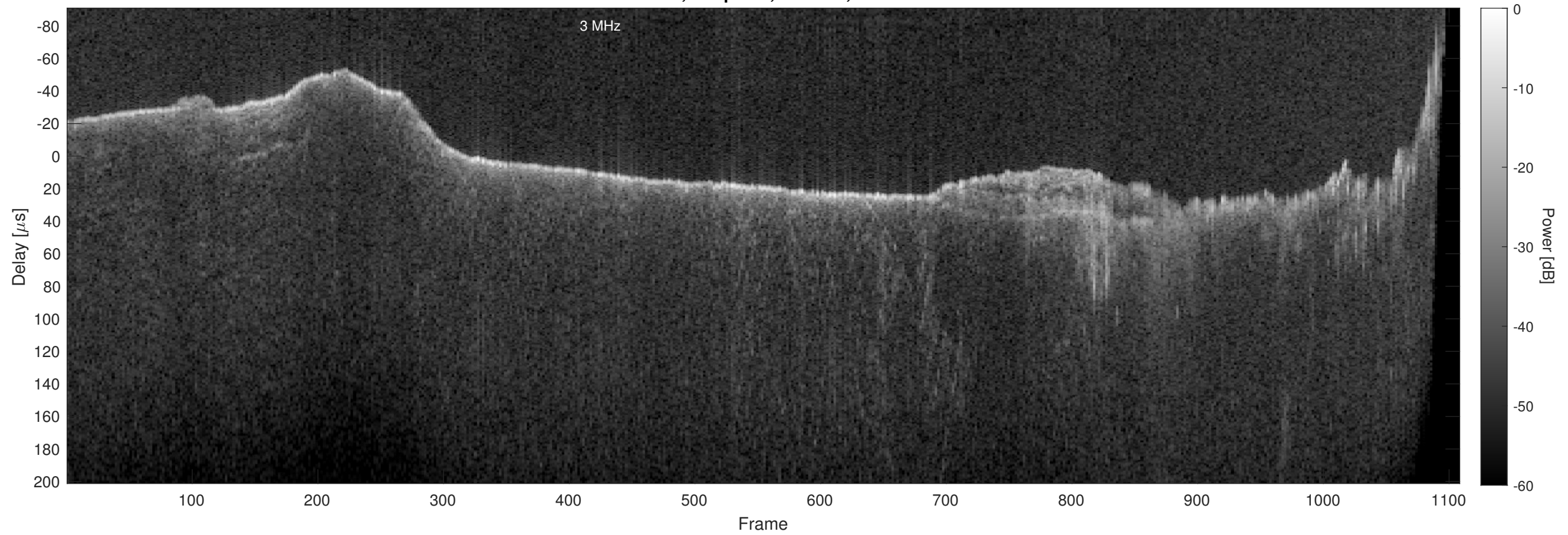
Orbit 14090, Chapman, Window, Channel 2
